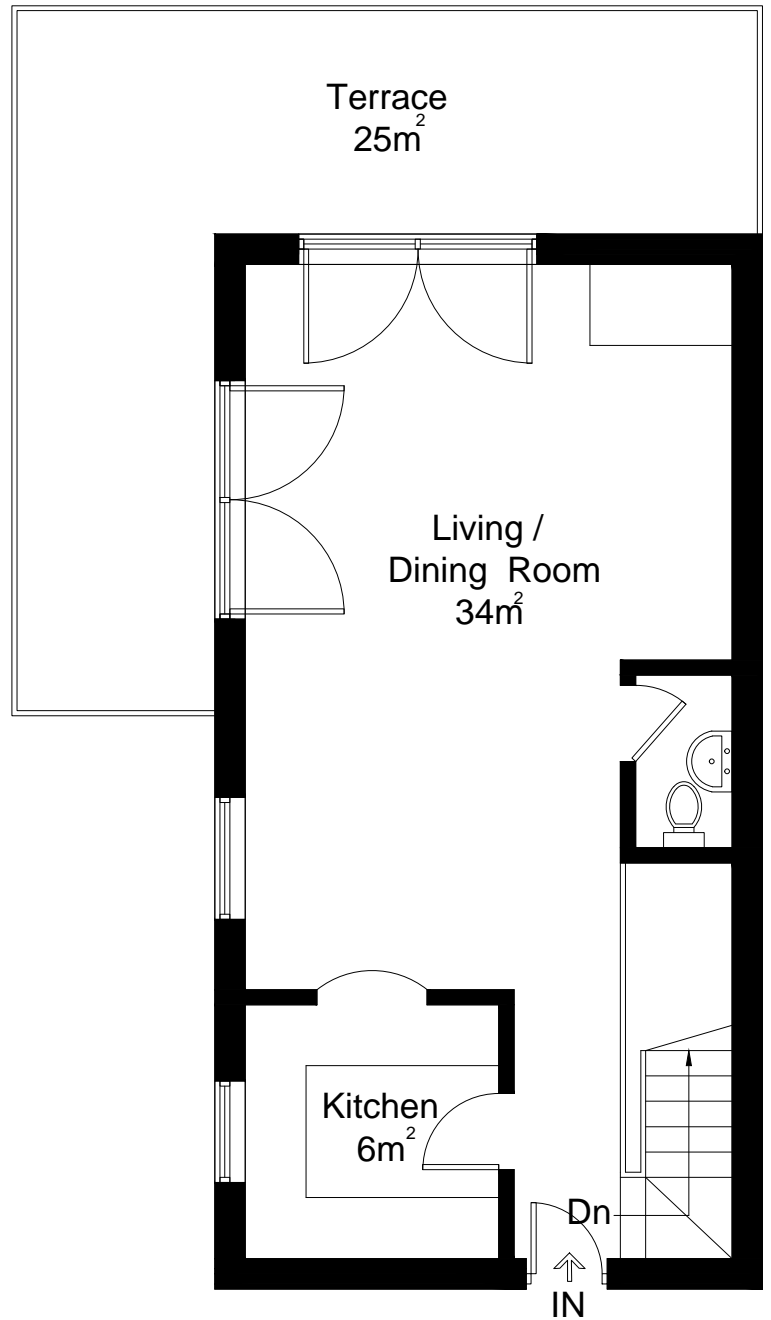
Ground Floor
